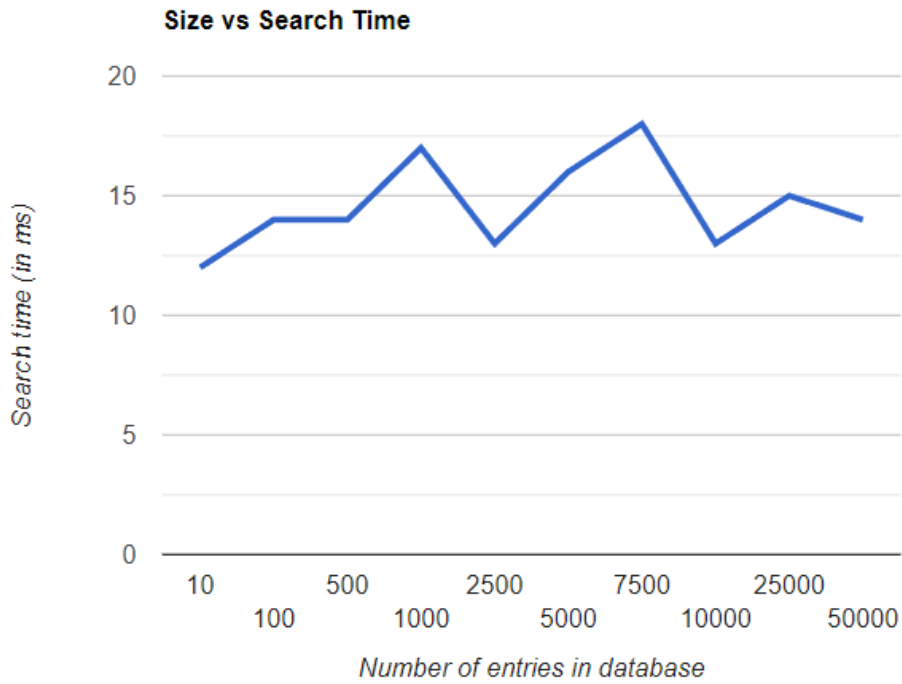
Figure 4: Graph showing how number of entries in a database affect the search time.
