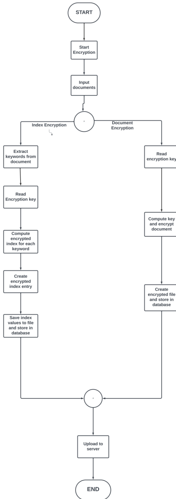
Figure 3: Flowchart explaining the index and document encryption process.
