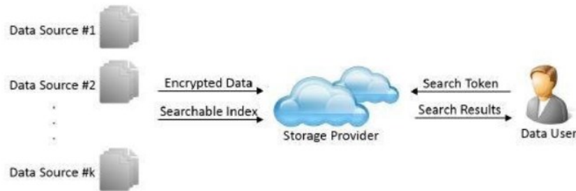
Figure 1: General SSE architecture where encrypted data is stored in the cloud and returns data when user queries after searching on encrypted data.
