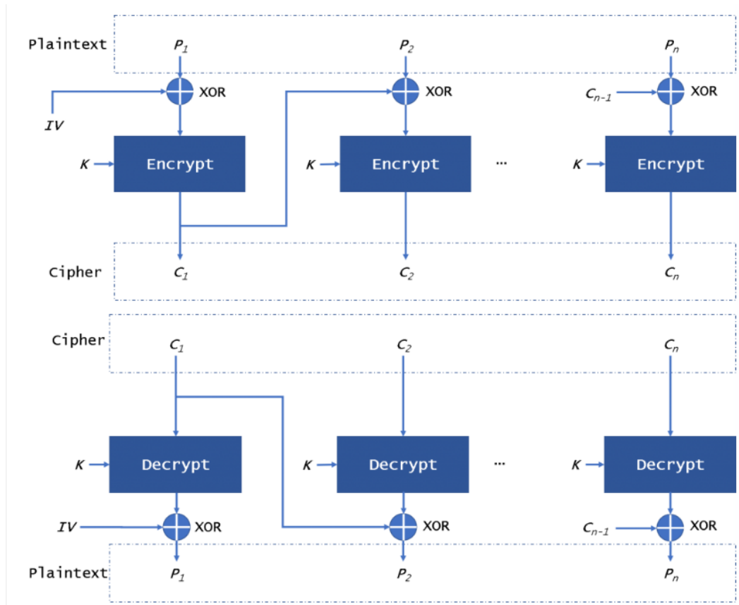
Figure 2: Working of AES in CBC mode
