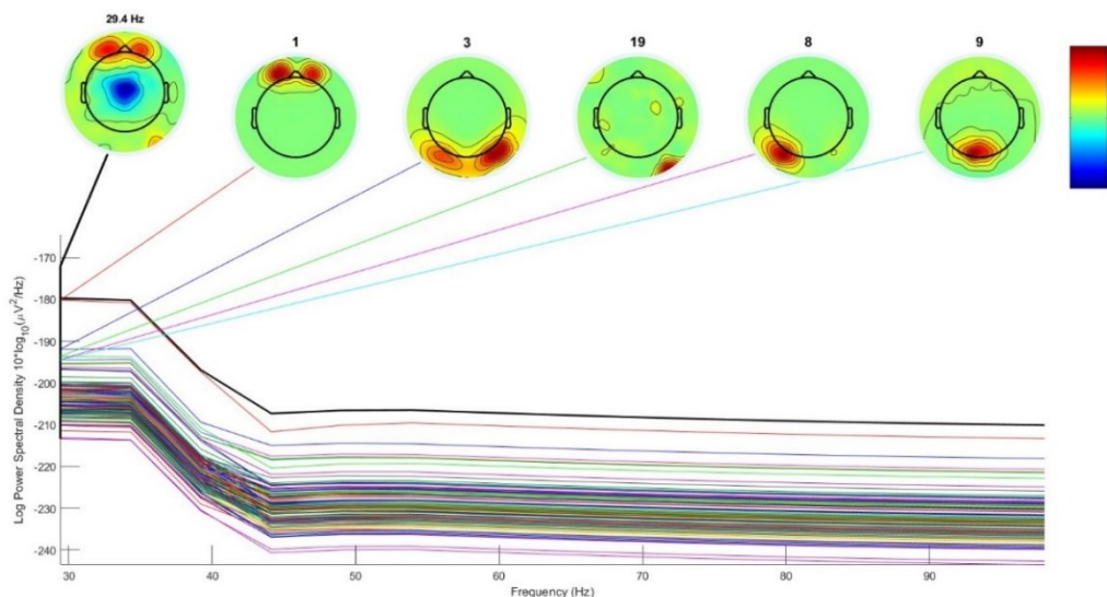
Figure 2 Gamma Bands 30 Hz 200 to 300ms
