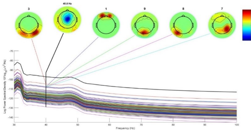
Figure 3 Gamma Bands 40 Hz -1000ms to 1996ms
