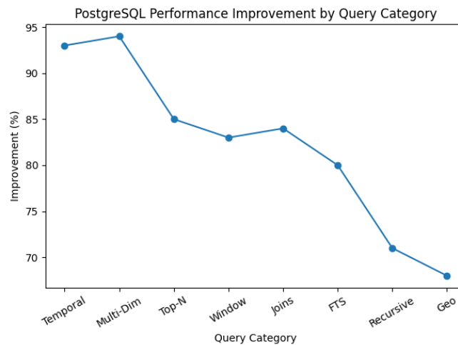
Figure 6. Performance Improvement by Query Pattern Category on PostgreSQL
