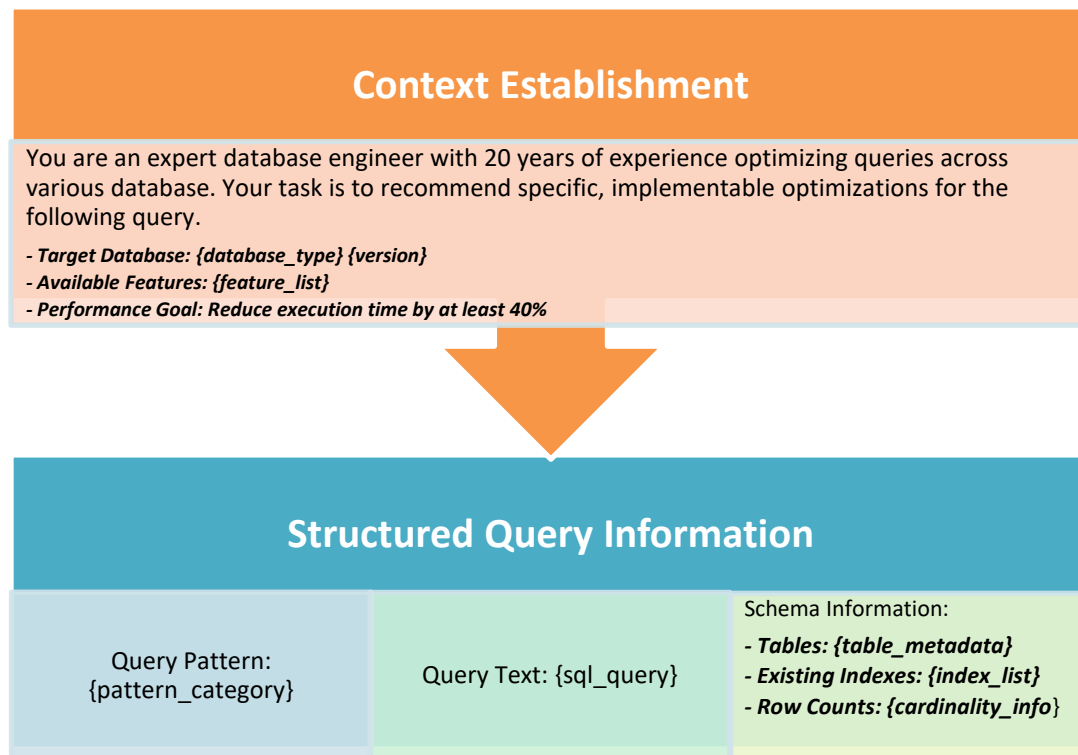
Figure 2. Stages in LLM Recommendation Engine
