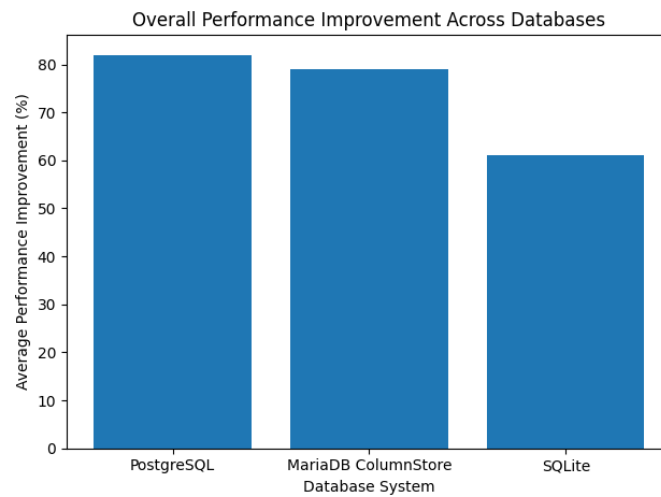
Figure 5. Average Performance Improvement Across Database Systems Over 16 Query Test Cases
