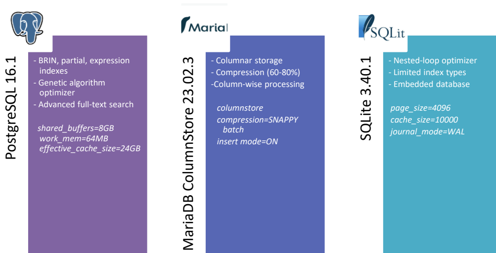
Figure 4. Key Features and Configuration on the Selected Database Systems
