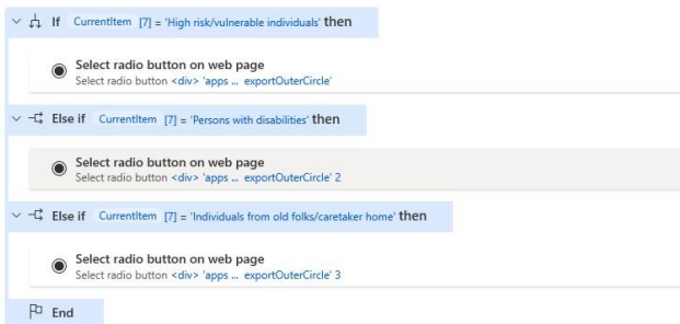
Figure 21. If else statements for Radio Buttons
