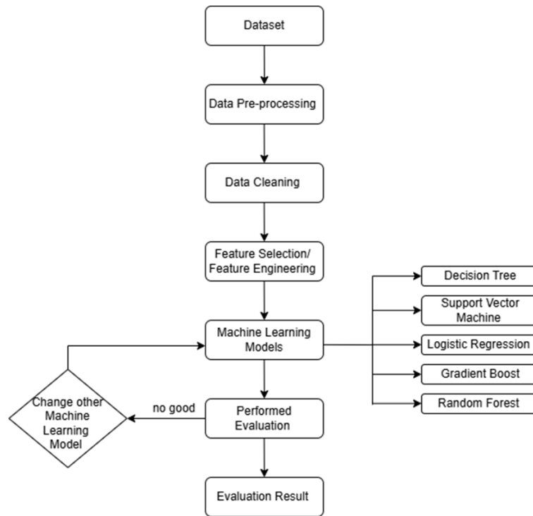
Figure 1. Propose Framework
