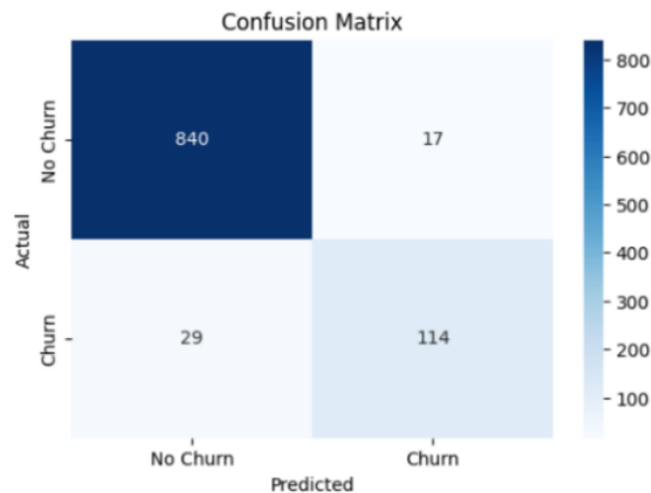
Figure 2. Confusion Matrix of RF Classifier in Dataset 1
