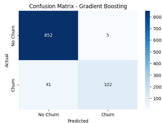
Figure 10. Confusion Matrix of GB Classifier in Dataset 1
