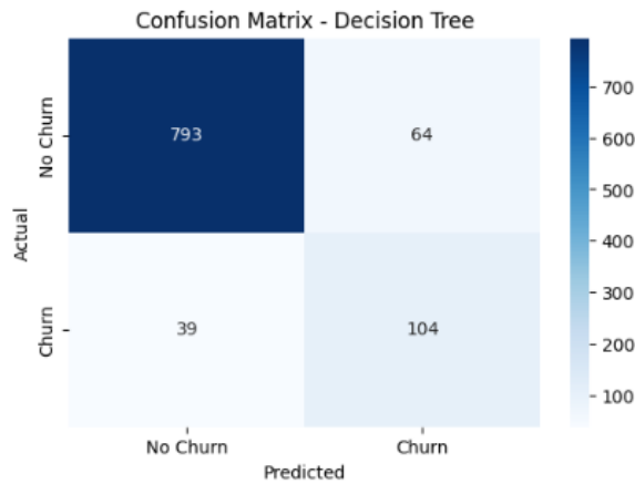
Figure 6. Confusion Matrix of DT Classifier in Dataset 1
