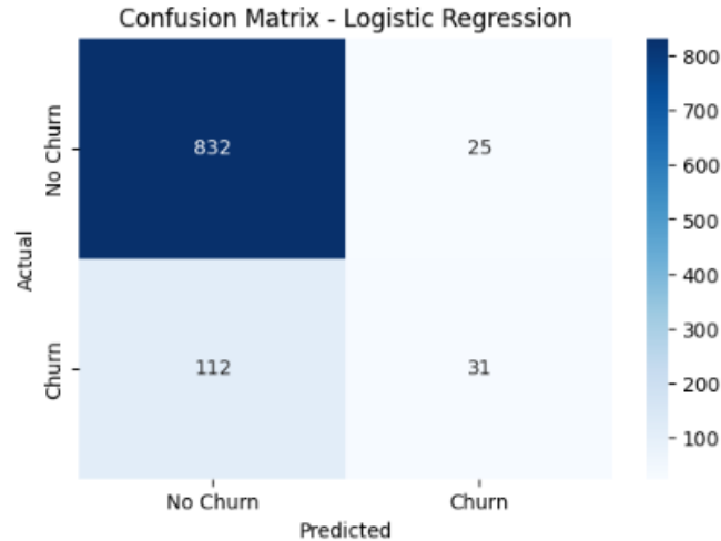
Figure 4. Confusion Matrix of LR Classifier in Dataset 1
