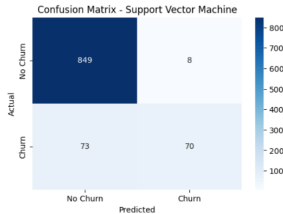
Figure 8. Confusion Matrix of SVM Classifier in Dataset 1
