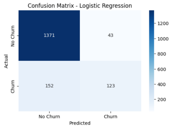
Figure 5. Confusion Matrix of LR Classifier in Dataset 2
