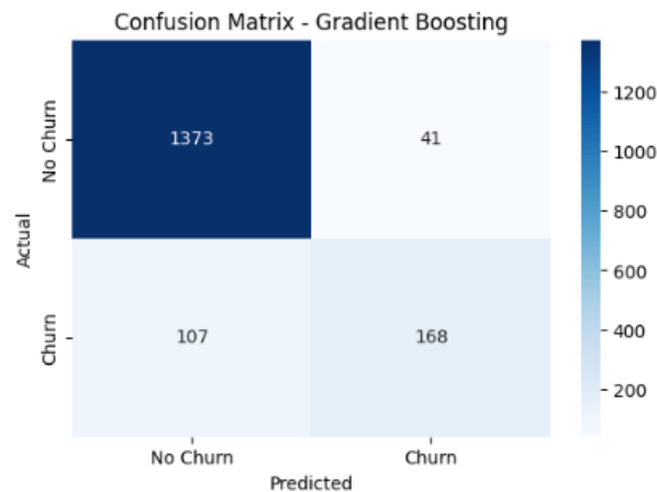
Figure 11. Confusion Matrix of GB Classifier in Dataset 2
