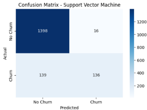
Figure 9. Confusion Matrix of SVM Classifier in Dataset 2
