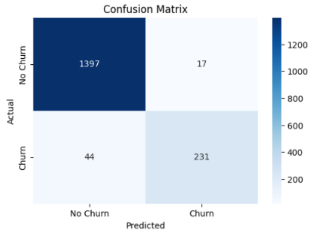
Figure 3. Confusion Matrix of RF Classifier in Dataset 2
