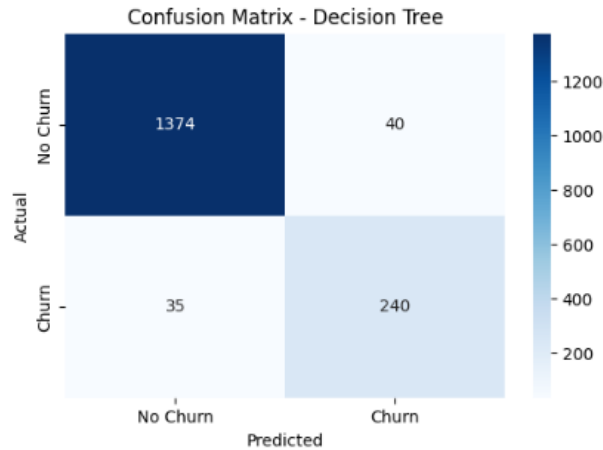
Figure 7. Confusion Matrix of DT Classifier in Dataset 2
