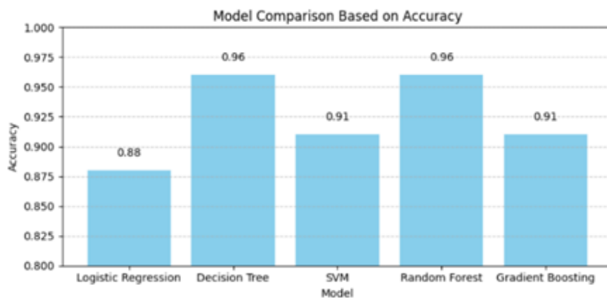
Figure 13. Comparison of Model Accuracy in Dataset 2
