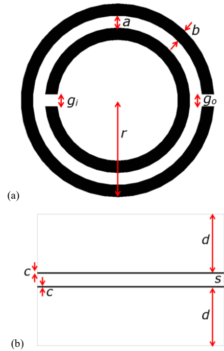
Fig. 3. Geometric structures of (a) the SRR and (b) the CPW used in the lock assemblies.
