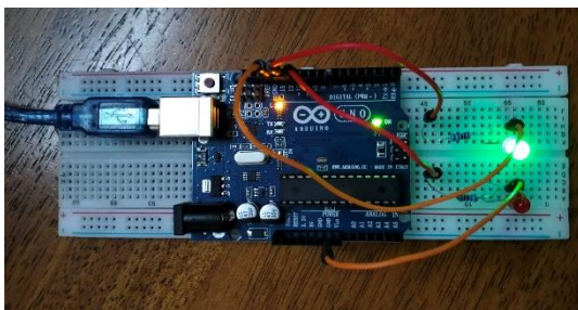
Fig. 6. Successful unlocking of the system with an SRR oriented at 30°; the green LED indicates that the measured resonant frequency and transmission dip match the stored configuration within the allowed tolerance.
