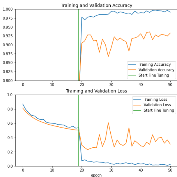
FIGURE 5. Accuracy and loss curve of ResNet101v2.
