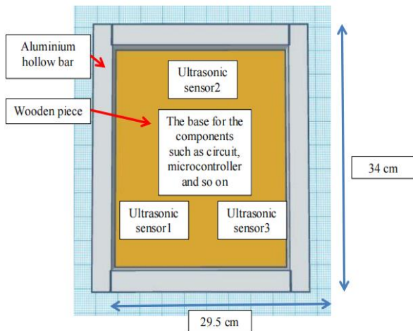
FIGURE 2. Top view of automatic solar grass trimmer.
