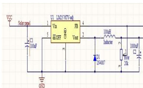
FIGURE 6(A). Schematic for dc - dc buck converter.
