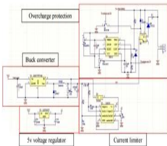
FIGURE 5. Solar charge control circuit.
