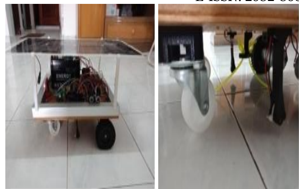
FIGURE 7(B). Tthe side and bottom view of the completed machine.
