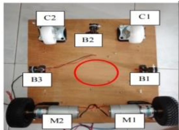
FIGURE 4(A) Bottom view.
