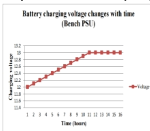
FIGURE 9(A). Charging voltage vs time (Bench PSU).
