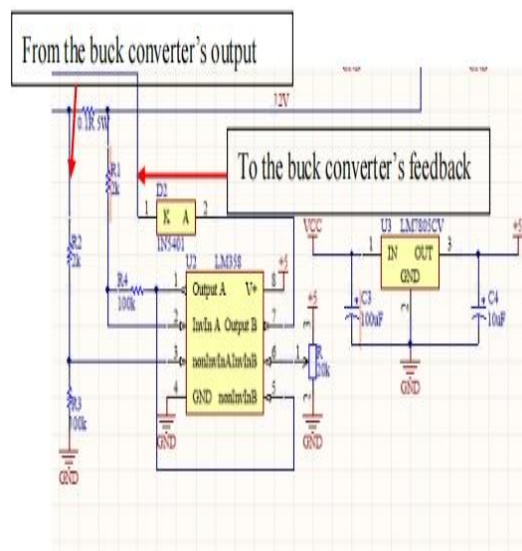
FIGURE 6(B). Schematic of current limiter circuit.
