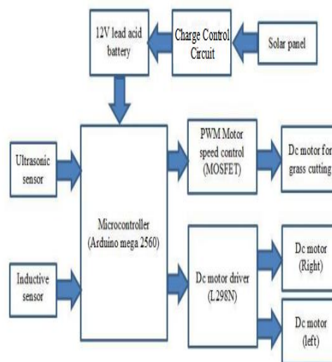
FIGURE 1: Block diagram of automated solar grass trimmer.
