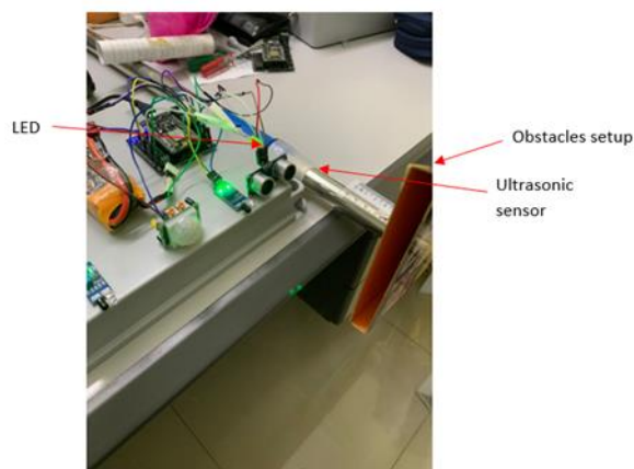
Figure 21. The setup of the experiment
