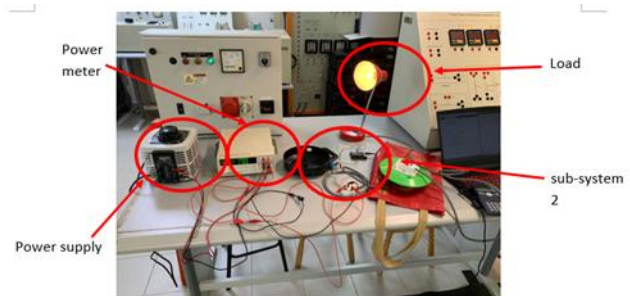
Figure 24. The setup of the experiment
