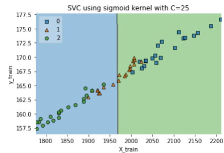
FIGURE 9. Decision boundary of sigmoid kernel with C = 25 .
