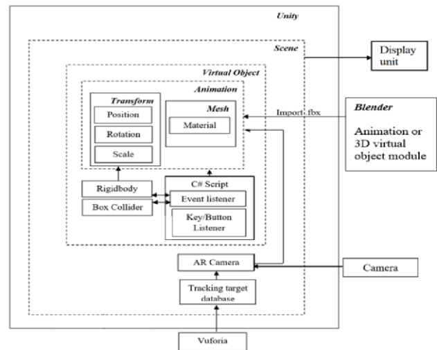
FIGURE 3. System configuration.
