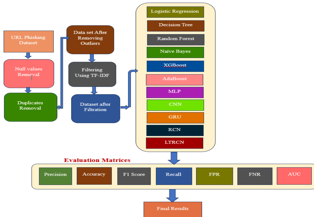
FIGURE 1. Classification of Phishing URL's Using ML and DL Models.
