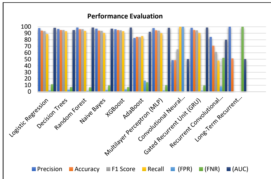
FIGURE 2. Experimental Results of Classification of Phishing URL's Using ML and DL Models
