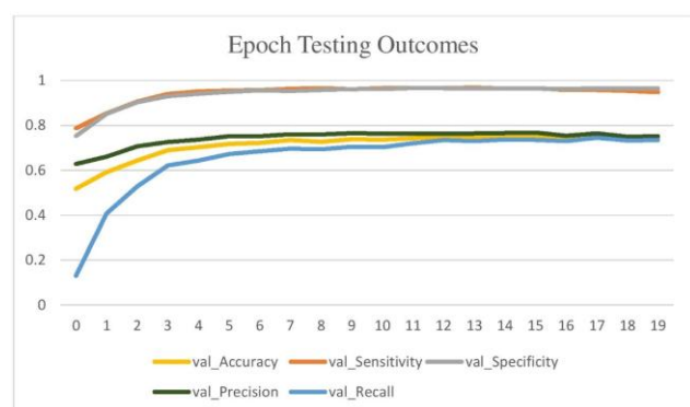
FIGURE 9. Testing performance of CNN classifier over multi epochs for customer sentiment.
