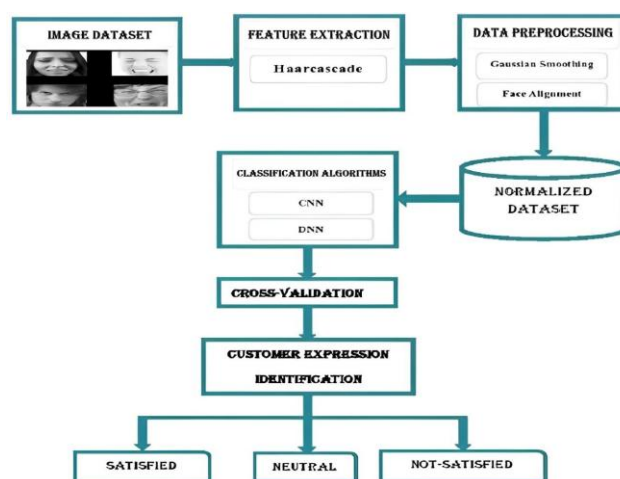
FIGURE 1. Proposed system framework.
