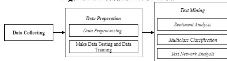
Figure 2: Research Workflow
